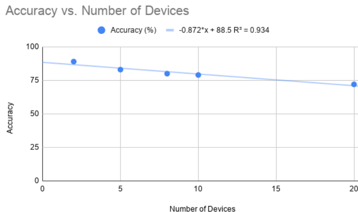
Figure 4: Accuracies of SVMs vs Number of Devices Trained and Tested On.
